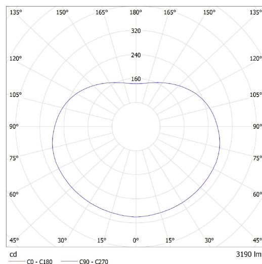
Lucis ZKS.L1.400.X POLARIS ZKS LED / LDC (Polar)
